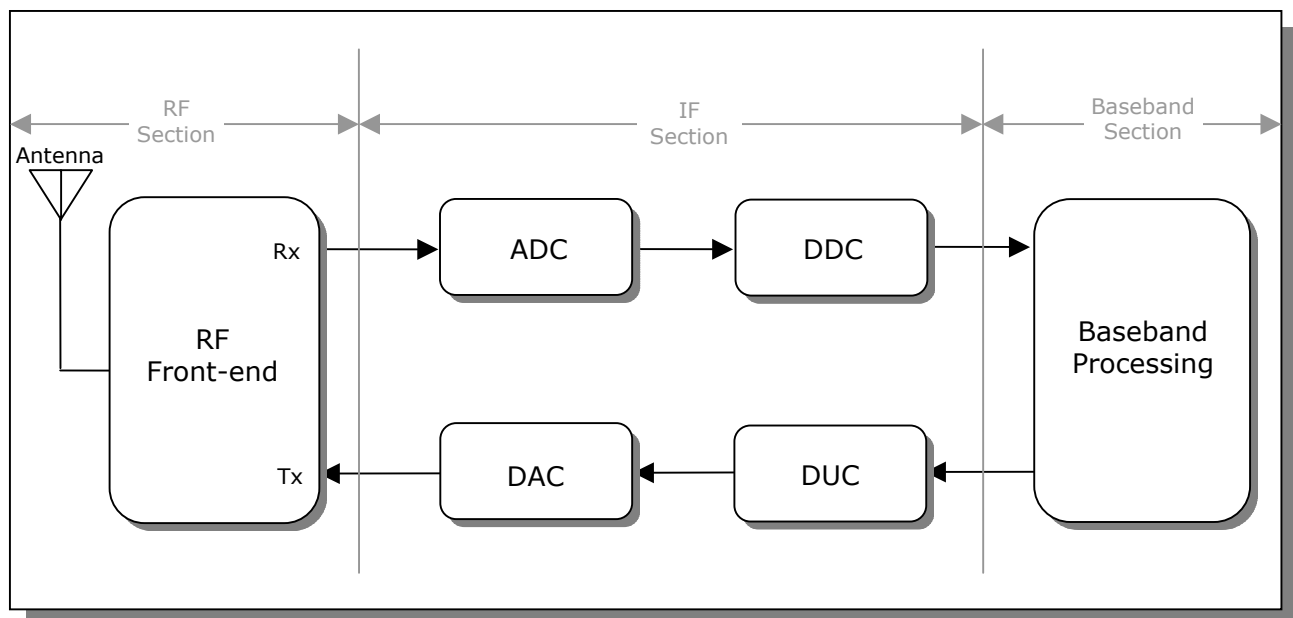
Figure 1: Block diagram of a generic digital transceiver
