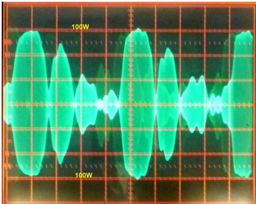
Figure 4: SSB RF envelope at 100W PEP. Note ALC compression on voice peaks.
