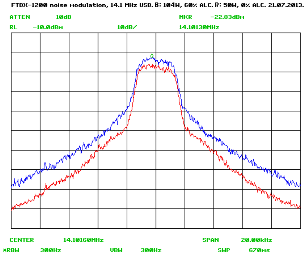
Figure 9: Spectrogram of Gaussian noise at 104W & 50W PEP, showing IMD skirts.
